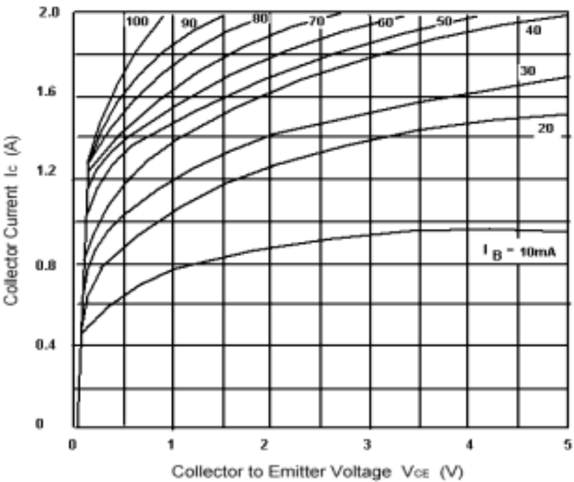
Fig.4 Static Characteristic
