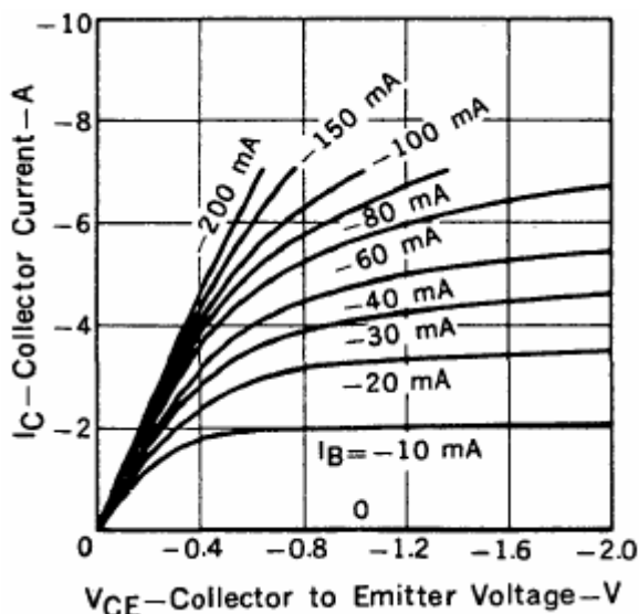
Fig.3 Static Characteristic
