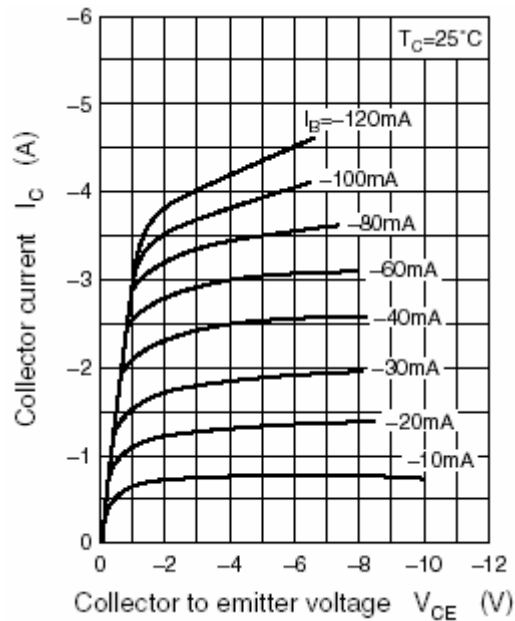
Fig.3 Static Characteristic
