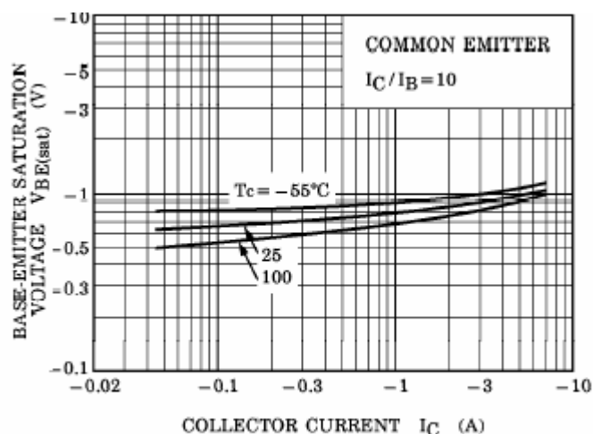
Fig.6 Base-Emmitter Saturation Voltage
