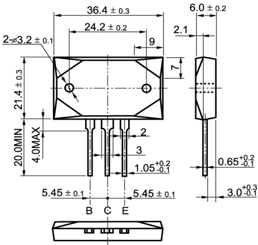
Fig.2 Outline dimensions
